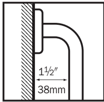
Clearance between wall and grab bar.
